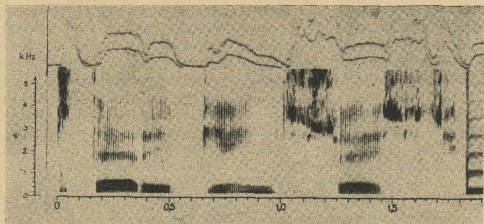
Fig. 2. 'Sonagram' and 'amplitude display' (two overall level curves) of the words cztery, pięć, sześć /tʃteri | pjentɕ | fectɕ/. Note: (1) Pulse-like segments for /t/ and /p/ in /tʃteri/ and /pjentɕ/. (2) A pulse-like segment followed by noise for /tɕ/ in /pjentɕ/. (3) A longer and a shorter noise segment for /ɕ/ and /tɕ/ in /fectɕ/ with another, weak noise segment in between, and no pulse for the affricate.
