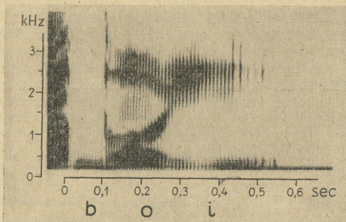
Fig. 5. 'Sonagram' of the word /boi/. Note: /i/ extends from 0.27 sec. to 0.53 sec — duration 0.25 sec.
