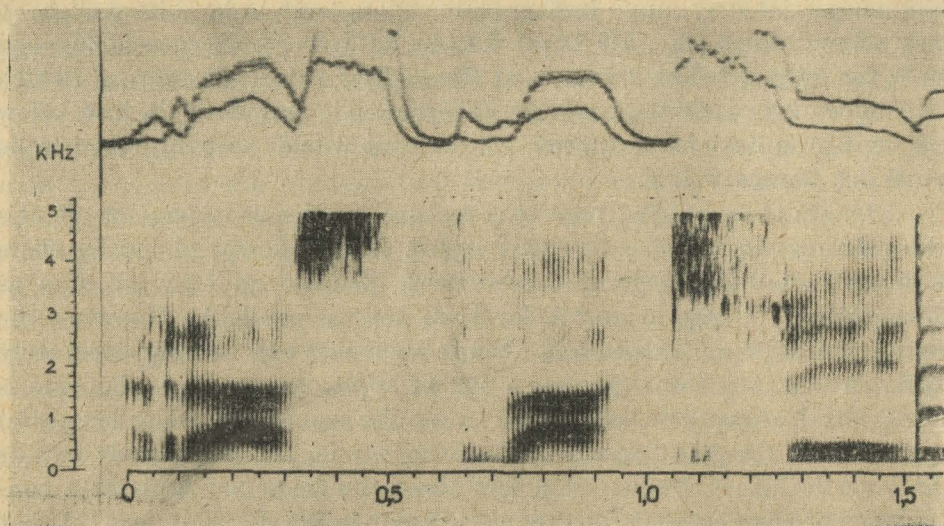
Fig. 1. 'Sonagram' and 'amplitude display' (two overall level curves) of the words raz, dwa, trzy /ras | dva | tʃʃi/. Note: (1) A succession of two quick 'dips' in the overall level curve and the corresponding two short weakenings of the spectrographic pattern for the /r/ in /ras/. (2) A quick up-and-down of the overall level curve for the plosion of /d/. (3) A trace of a pulse-like segment followed by wide-band noise for /tʃʃ/ in /tʃʃi/.
