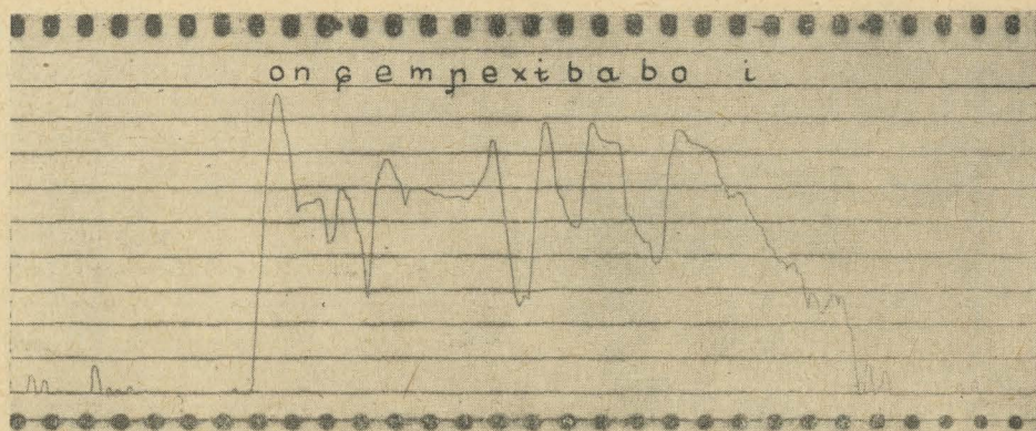
Fig. 3. Overall level curve (taken with a Bruel and Kjaer level recorder — dynamic range 25 db) of the sentence On się mnie chyba boi.
