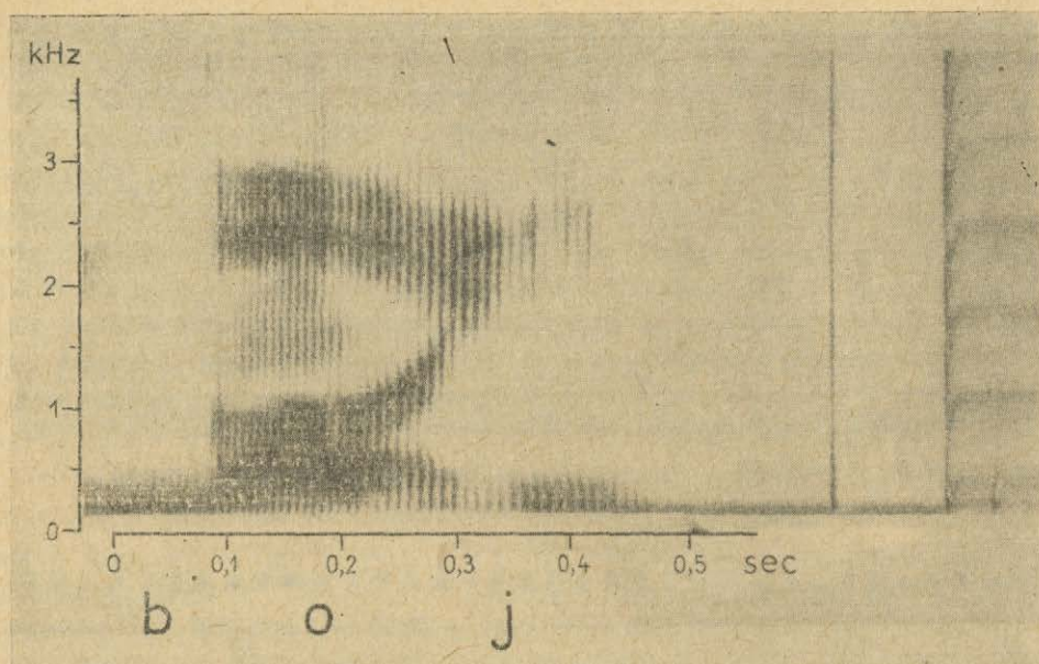
Fig. 6. 'Sonagram' of the word /boj/. Note: /j/ extends from 0.30 sec. to 0.46 sec. — duration 0.16 sec.
