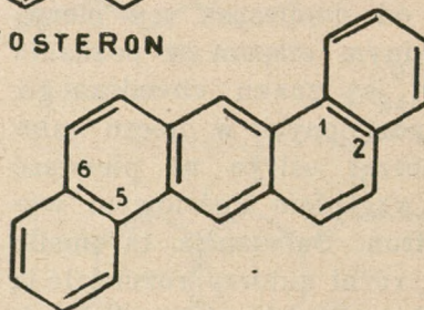
1,2,5,6-DWU-BENZANTRACEN
