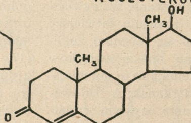
TESTOSTERON
